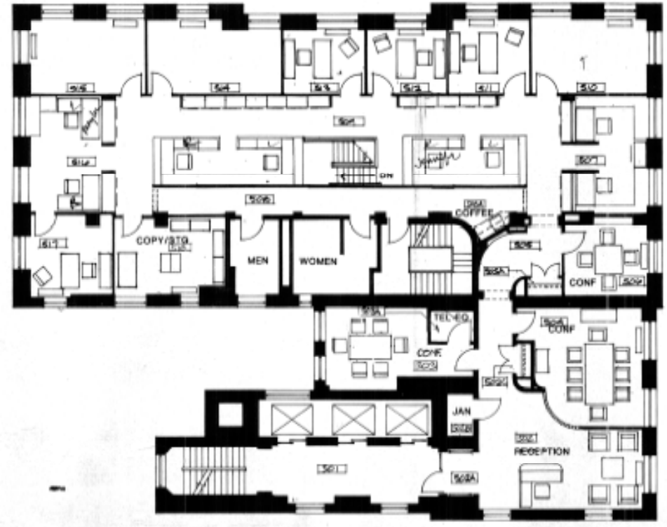
1 5th FLOOR PLAN
